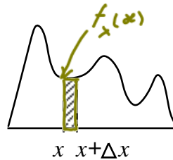
Figure 27: P[x \leq X \leq x + \Delta x] is the area of the shaded vertical strip.
